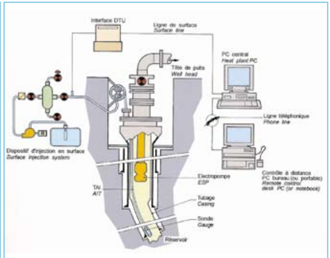
● Combined chemical injection/control line set up
